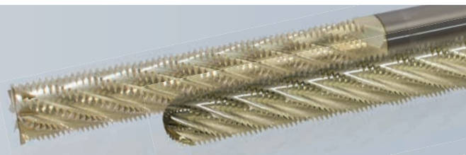
29-100 Series Diamond Grit Hogger Solid Carbide Honeycomb Hogger Product Offering
