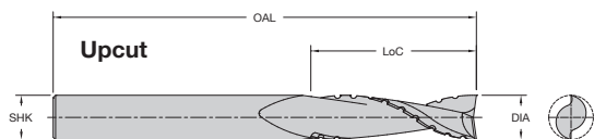
60-300 Series Two Flute - Solid Carbide Chipbreaker Finisher ( Upcut ) Product Offering
