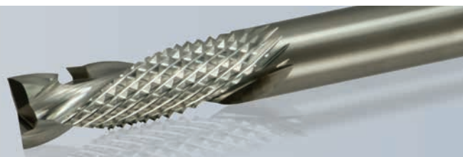
67-400 Series Solid Carbide Un-Ruffer™ PATENTED Product Offering
