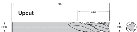
60-350 Series Three Flute - Solid Carbide Chipbreaker Finisher ( Upcut ) Product Offering
