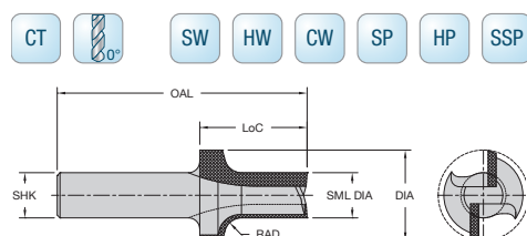
40-50 Series Two Flute - Carbide Tipped Lettering Bits Product Offering
