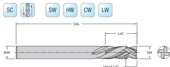
60-600 Series Four Flute - Solid Carbide High Velocity Compression Spiral Product Offering
