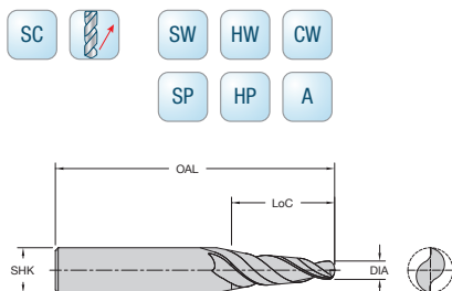
77-100 Series Two or Three Flute Solid Carbide Taper Tools Product Offering
