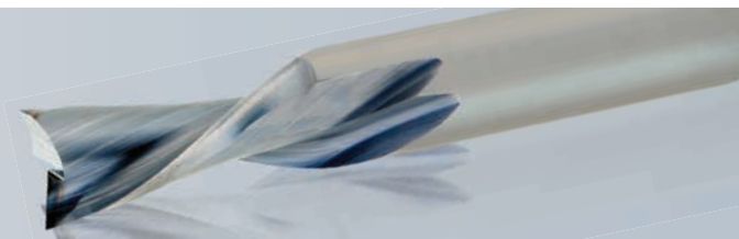
57-400 Series Two Flute - Solid Carbide Downcut Spiral Wood Rout Product Offering - Metric
