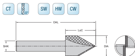
37-80 Series Two Flute - Carbide Tipped Lettering Bits Product Offering
