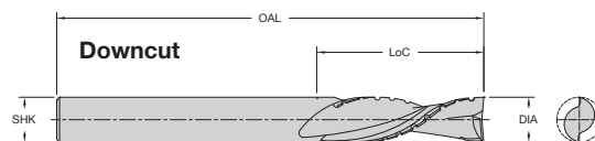
60-300 Series Two Flute - Solid Carbide Chipbreaker Finisher ( Downcut ) Product Offering
