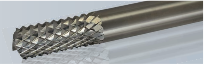
67-000 Series Solid Carbide Fiberglass Router Medium Burr W/End Mill Point Product Offering
