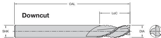
60-350 Series Three Flute - Solid Carbide Chipbreaker Finisher ( Downcut ) Product Offering
